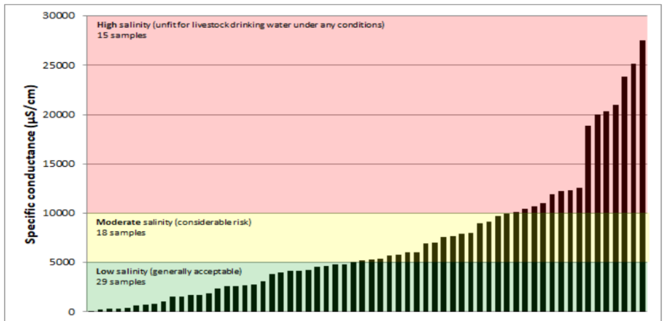
Figure 22. Petroleum County livestock pond 2020 sampling results showing number of samples falling in ranges of low (green), moderate (yellow) and high (pink) salinity (Hauschild, 2020).
